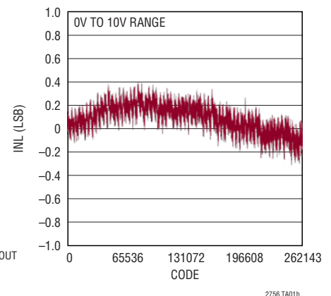
LTC2756 Integral Nonlinearity
